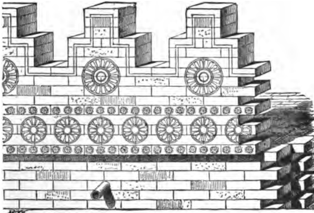
53.—BATTLEMENTS OF THE TERRACE WALL AT DUR-SHARRUKIN, AND DRAIN PIPE. (RESTORED FROM FRAGMENTS FOUND ON THE SPOT.)
